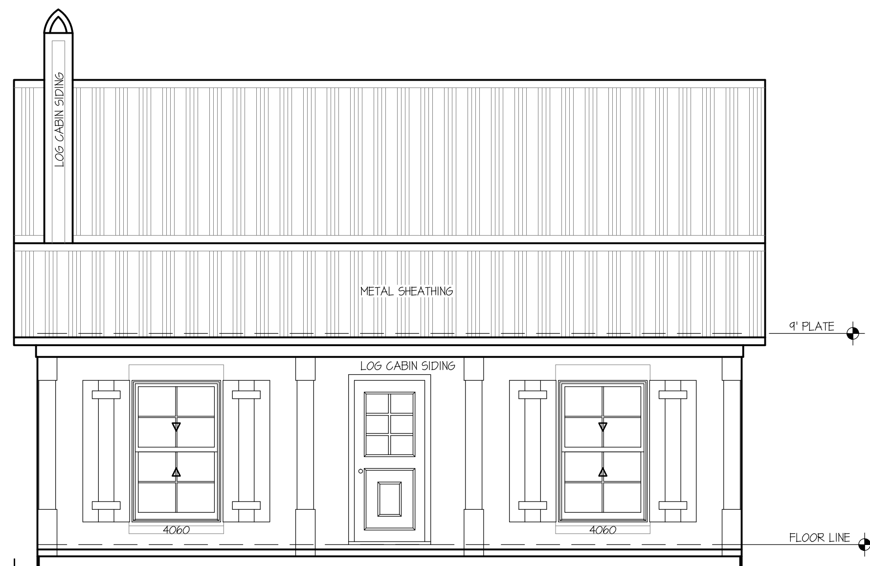
FRONT ELEVATION
