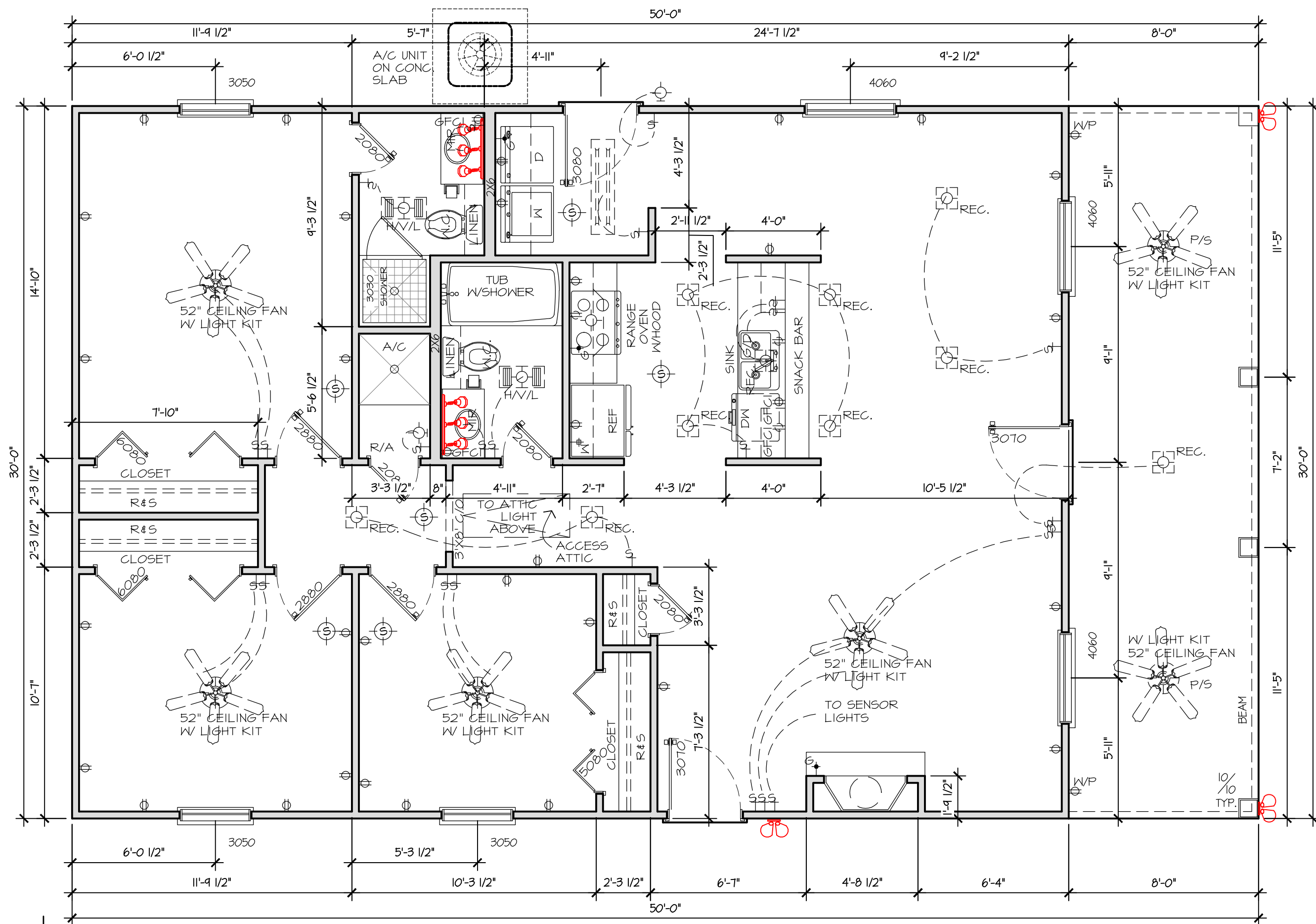
FLOOR PLAN
