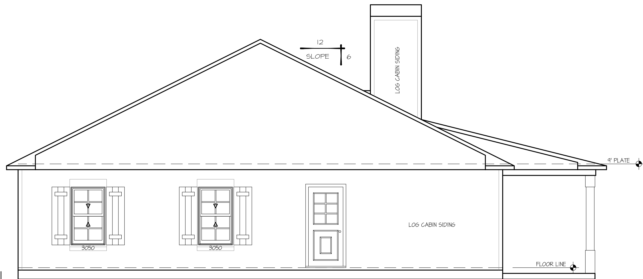
LEFT ELEVATION
